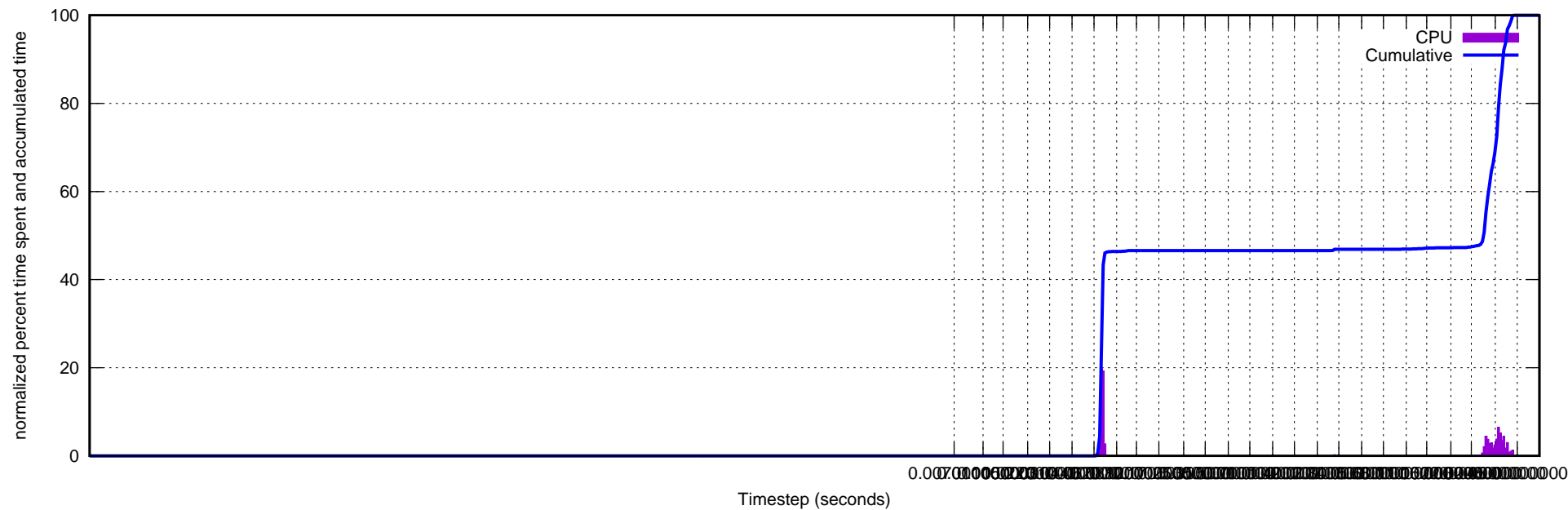
CPU Time Step Statistics for dir.logs/jr-ens06-1004.log.gz
