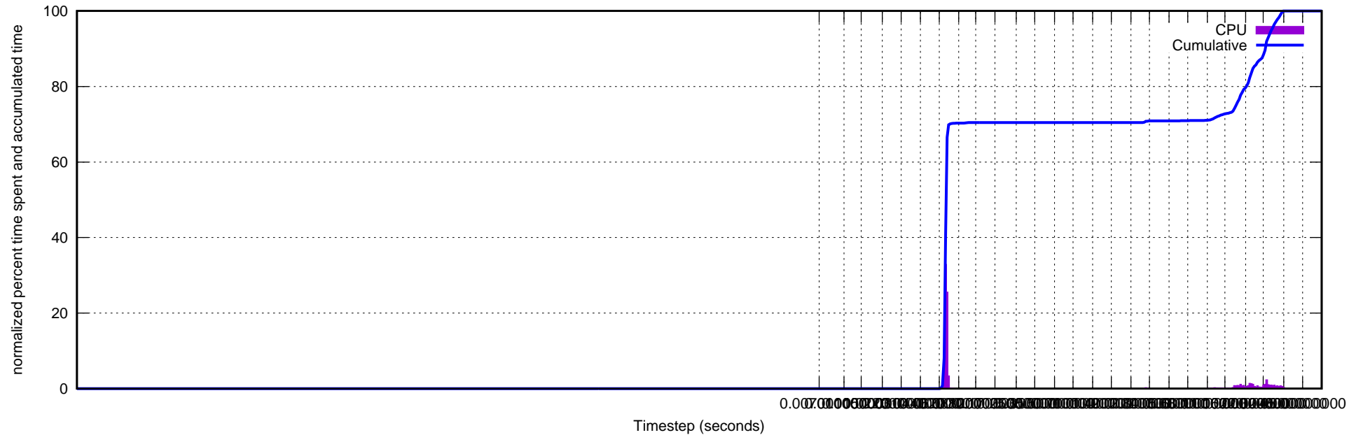
CPU Time Step Statistics for dir.logs/jr-ens06-1003.log.gz
