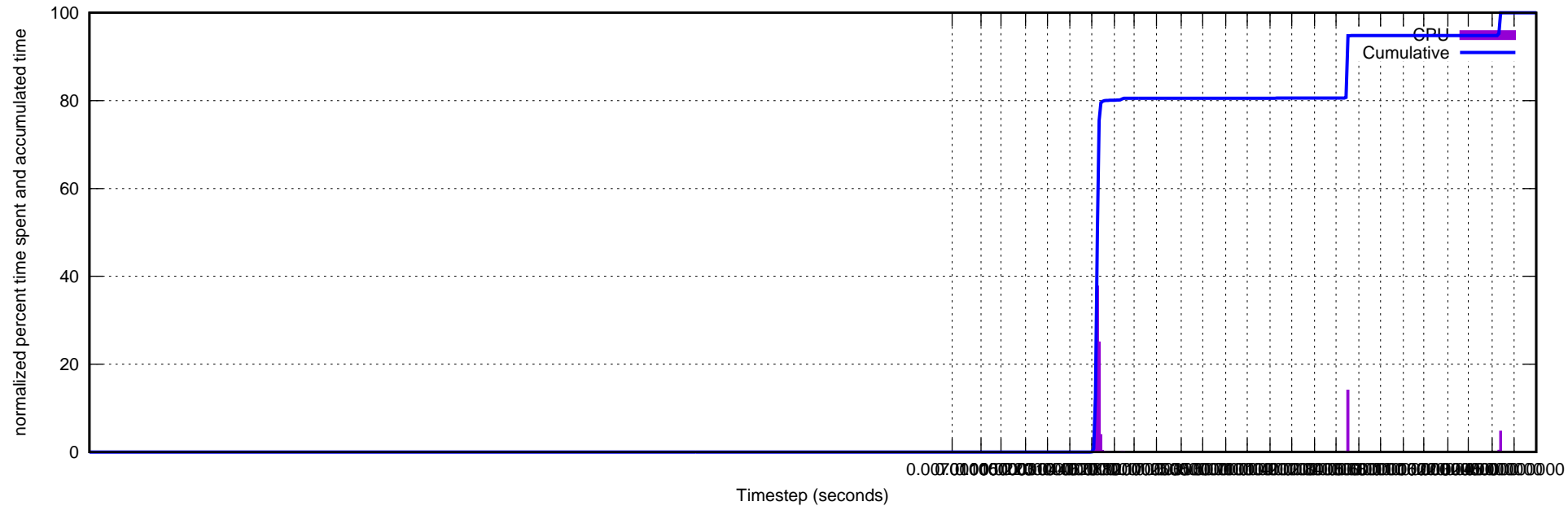
CPU Time Step Statistics for dir.logs/jr-ens03-1001.log.gz
