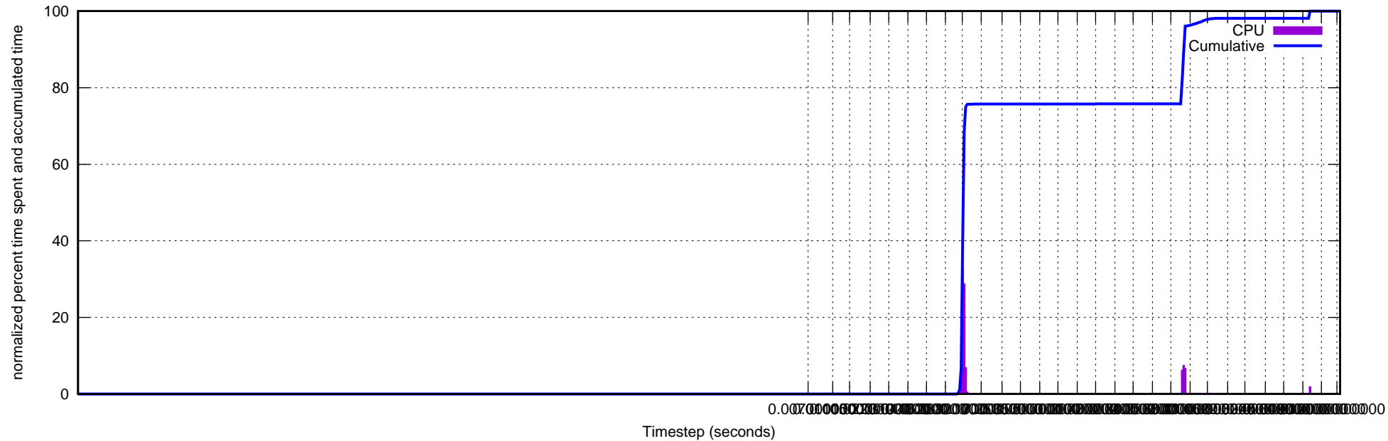
CPU Time Step Statistics for dir.logs/jr-2015-03-15.log.gz
