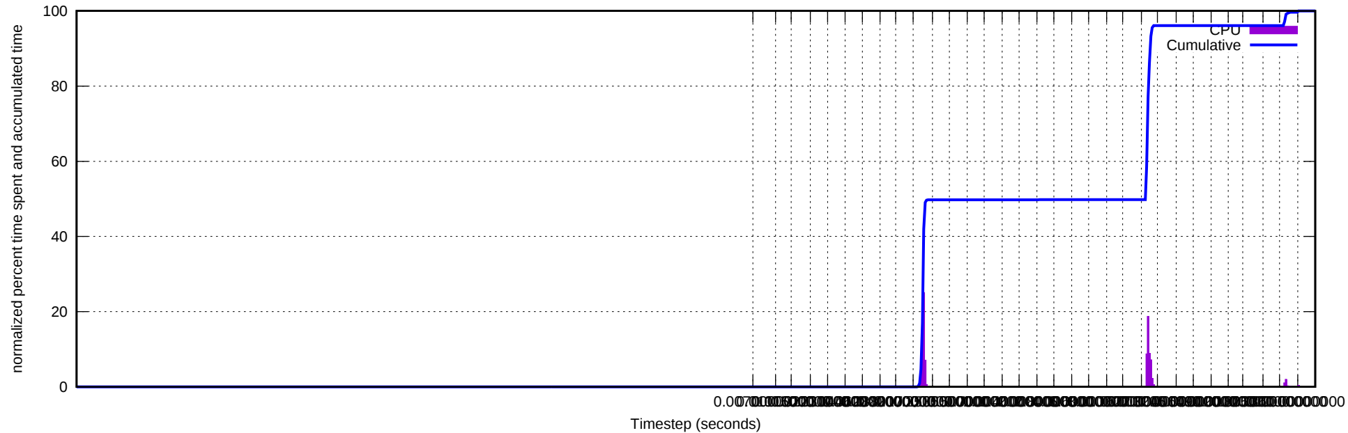
CPU Time Step Statistics for dir.logs/jr-2009-01-03-f3.log.gz
