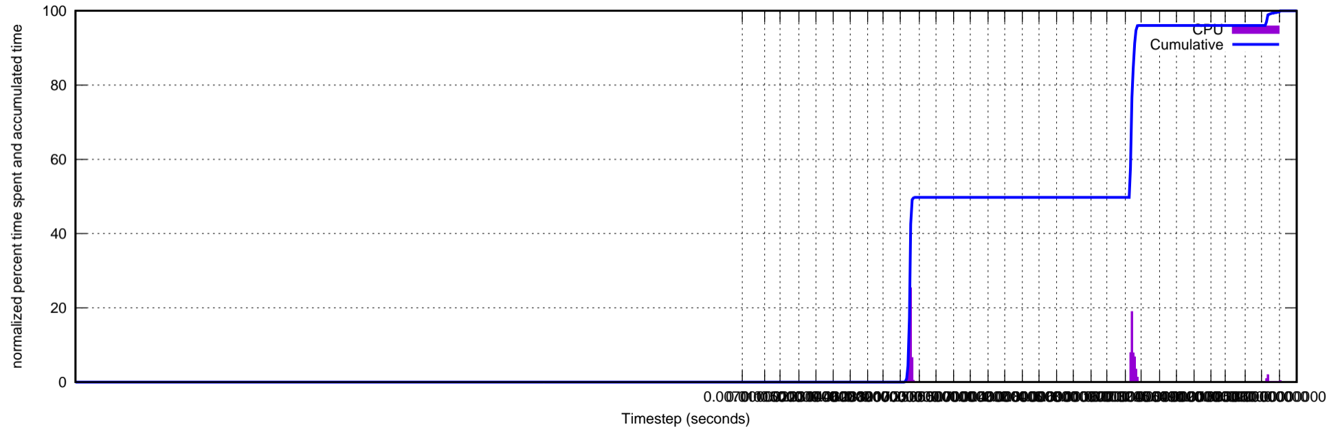
CPU Time Step Statistics for dir.logs/jr-2009-01-03-f1.log.gz
