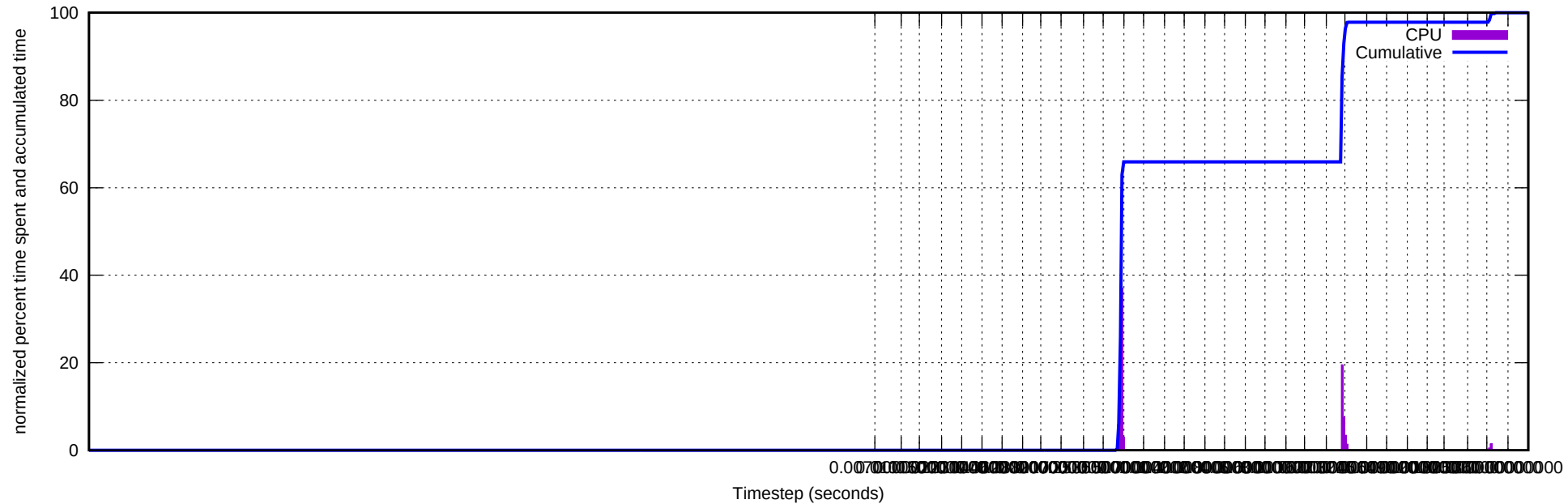
CPU Time Step Statistics for dir.logs/jr-2009-01-03-e7.log.gz
