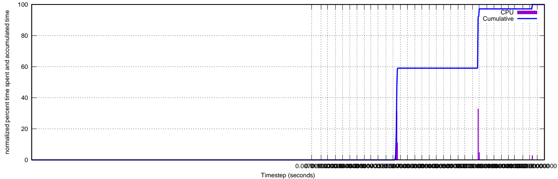
CPU Time Step Statistics for dir.logs/jr-2009-01-03-e4.log.gz
