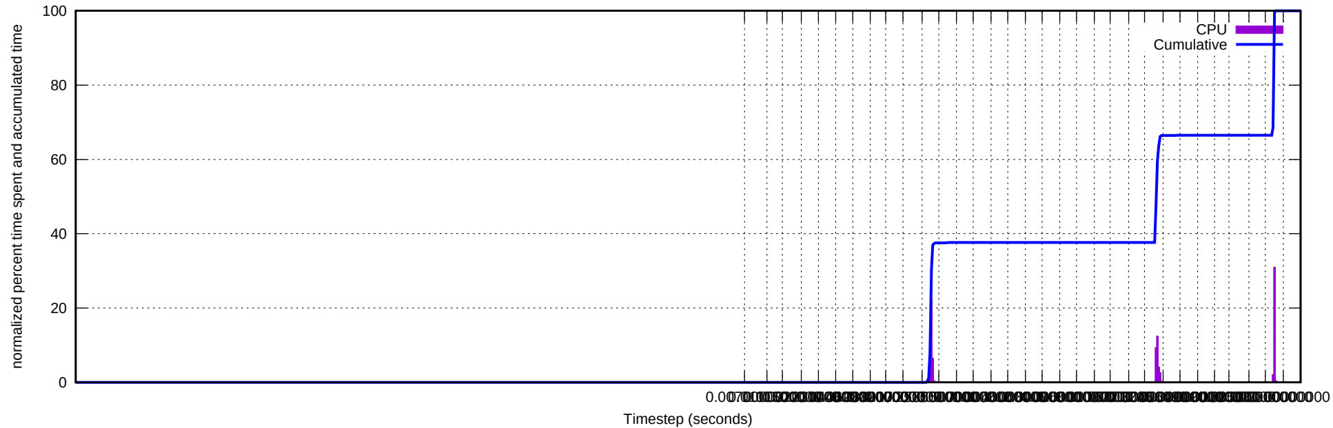
CPU Time Step Statistics for dir.logs/jr-2009-01-03-d4.log.gz
