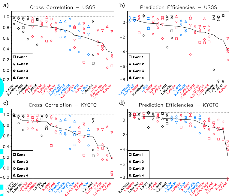
Figure 5. Model ranking using Correlation Coefficient ( CC ) and Prediction Efficiency ( PE ).
