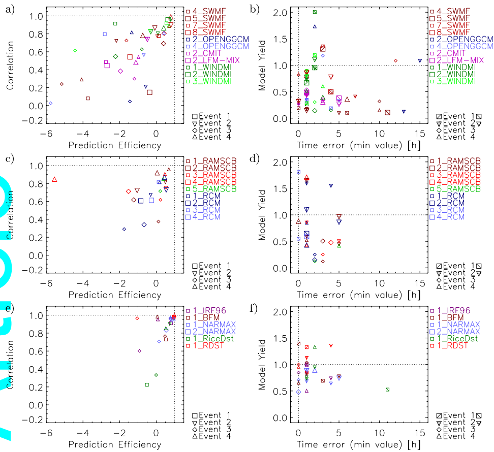
Figure 7. Model runs in 2D skill score space. Prediction Efficiency ( PE ) and Correlation Coefficient ( CC ) are shown in Panels a), c), and e), left, with Panels a) and c) using USGS D_{st} values and Panel e) using KYOTO D_{st} values. In the right column, Timing Error ( \Delta T ) of minimum D_{st} value and Model Yield ( YI ) based on Kyoto D_{st} are shown in Panels b), d), and f). The top Panels, a) and b), show magnetosphere models, the middle Panels, c) and d), show ring current models, and the bottom Panels, e) and f), show D_{st} -specification models. Model runs are listed on the top right in each panel with a sample symbol for Event 1 shown. The color scheme is the same as in Figure 2. Runs that share a color are distinguished by symbol size. Each model setting may be run for up to 4 events, symbolized by a square for Event 1, a triangle pointing down for Event 2, a diamond for Event 3 and a triangle pointing up for Event 4. Dashed lines in the plot (vertical for the X-axis score, horizontal for the Y-axis score) indicate perfect scores. Events 1 and 2 have been split to determine \Delta T .
