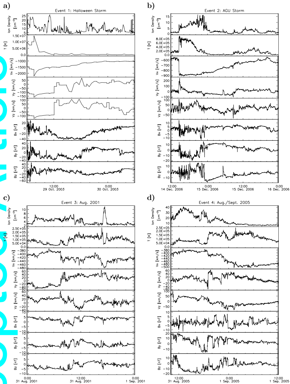
Figure 1. Solar wind bulk plasma and magnetic field observations for the four events listed in Table 1.
