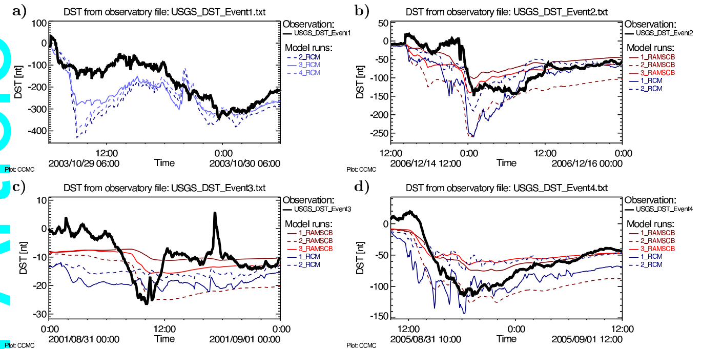
Figure 3. One-minute USGS D_{st} data (black line) and ring current model results (colors).
