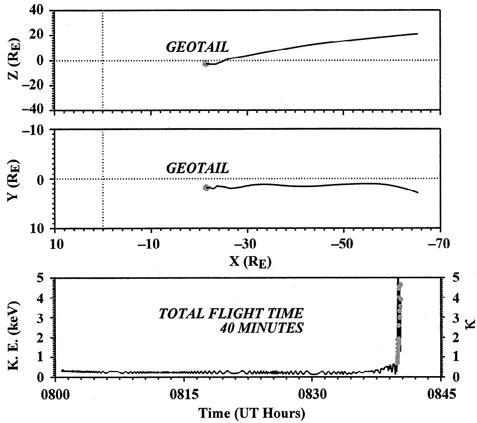
Figure 9. Trajectory of a northern plasma mantle particle reaching Geotail at 0840 UT in a similar format to that of Plate 1.
