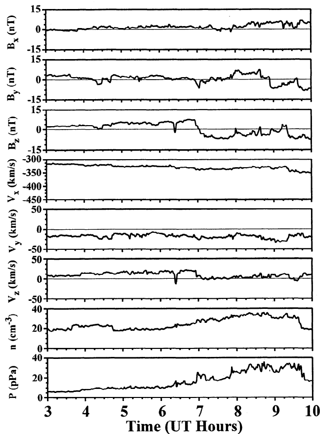
Figure 2. Wind data for November 24, 1996.
