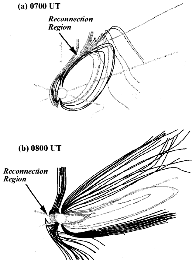
Figure 6. Field lines from MHD model for (a) 0700 UT (northward IMF) arrow indicates high-latitude reconnection region, (b) 0800 UT (southward IMF).
