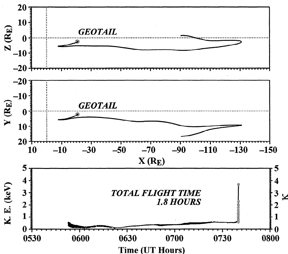
Figure 8. Trajectory of a duskside LLBL particle reaching Geotail at 0740 UT projected onto (a) x - z and (b) x - y planes. (c) Kinetic energy (black curve, scale on left) and \kappa (gray dots, scale on right) for the particle.
