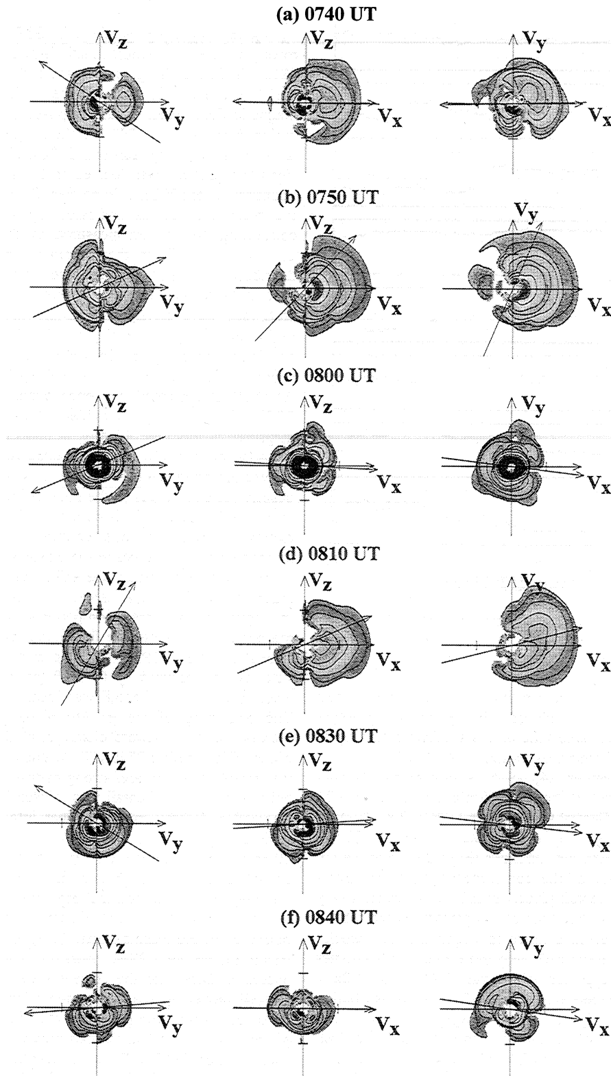
Figure 3. V_y - V_z , V_x - V_z , and V_x - V_y cuts of the Geotail distribution for six time intervals. (a) 0740, (b) 0750, (c) 0800, (d) 0810, (e) 0830, and (f) 0840 UT. Peak fluxes in the central parts of the distributions correspond to 2 \times 10^{-24} \text{ s}^3/\text{cm}^{-6} . The distributions are cut off at a flux level of 2 \times 10^{-26} \text{ s}^3/\text{cm}^{-6} .
