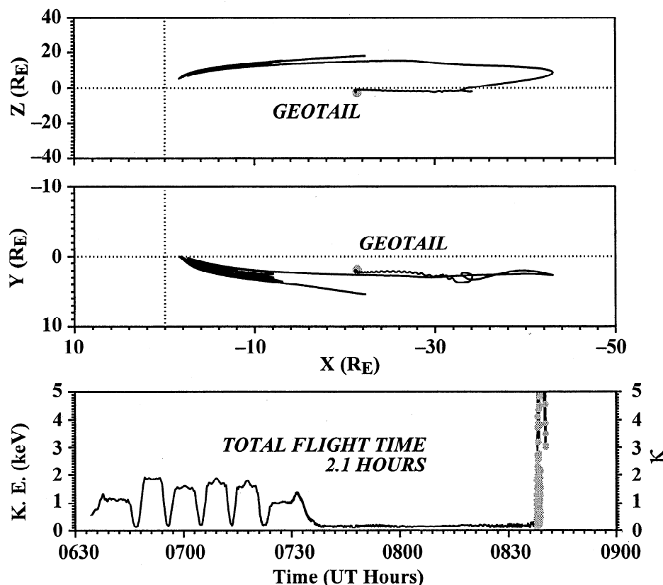
Figure 11. Trajectory of an ion entering through the high-latitude reconnection region and reaching Geotail at 0840 UT in a similar format to that of Plate 1.
