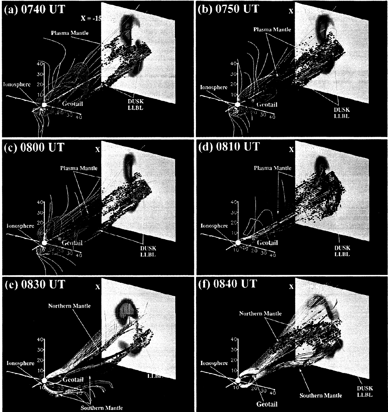
Plate 1. Magnetotail entry points for the ions in the Geotail distribution functions observed at (a) 0740, (b) 0750, (c) 0800, (d) 0810, (e) 0830, and (f) 0840 UT. Field line color coding is: red, closed; white, open; magenta, IMF.
