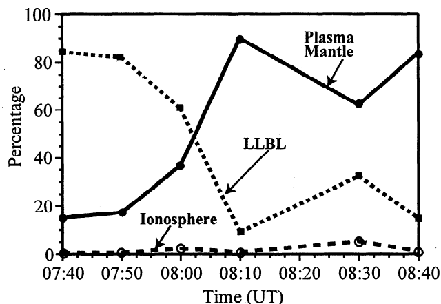
Figure 7. Percentage of ions measured by Geotail as a function of time that originate from the northern and southern plasma mantle (solid curve), the LLBL (dotted curve), and the ionosphere (dashed curve).
