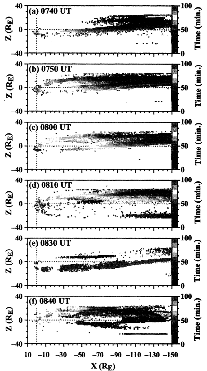
Plate 3. Projection of magnetotail entry points onto the x - z plane for the six time intervals: (a) 0740, (b) 0750, (c) 0800, (d) 0810, (e) 0830, and (f) 0840 UT. Color coding indicates the time of flight between the source and the point of measurement.
