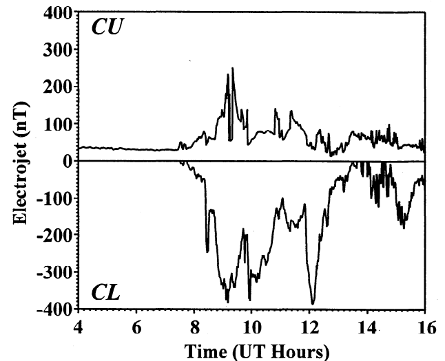
Figure 1. CANOPUS magnetometer data for November 24, 1996: (top) CU and (bottom) CL .
