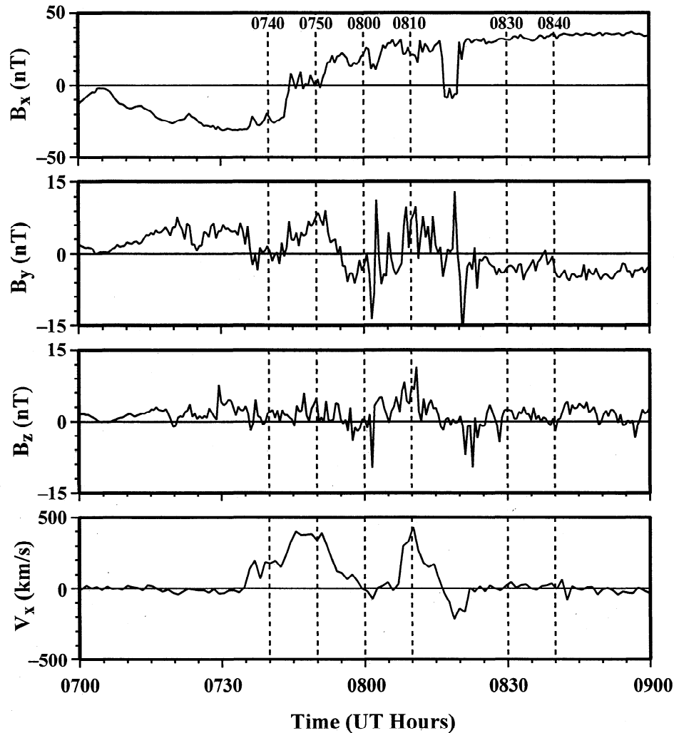
Figure 4. Geotail measurements in the magnetotail, showing profiles of (a) B_x , (b) B_y , (c) B_z , and (d) V_x .
