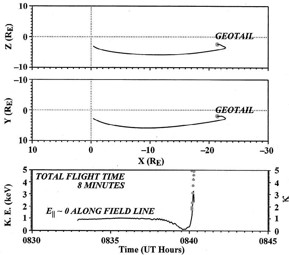
Figure 10. Trajectory of an ionospheric particle reaching Geotail at 0840 UT in a similar format to that of Plate 1.
