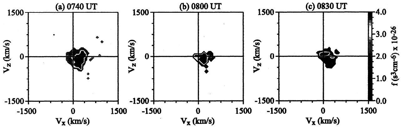
Plate 4. V_x - V_z Distribution of LLBL ions that reach Geotail at (a) 0740 UT, (b) 0800 UT, and (c) 0830 UT.
