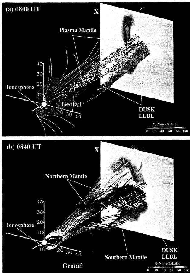
Plate 2. Magnetotail entry points for ions reaching Geotail at (a) 0800 and (b) 0840 UT. The color coding corresponds to the percentage of nonadiabatic ( \kappa < 2 ) ions in each 1 R_E^3 bin.
